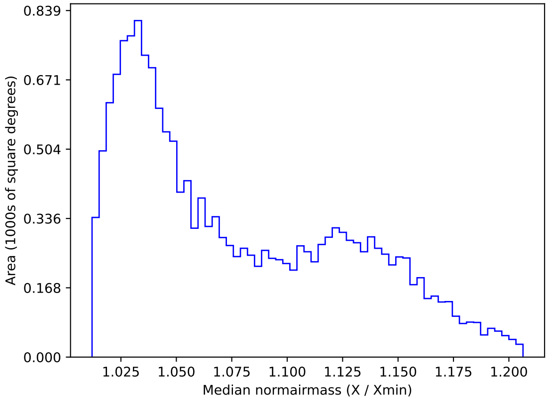
too_elab_r32_d3_gz_v3.4_10yrs WFD u band: Median normairmass
