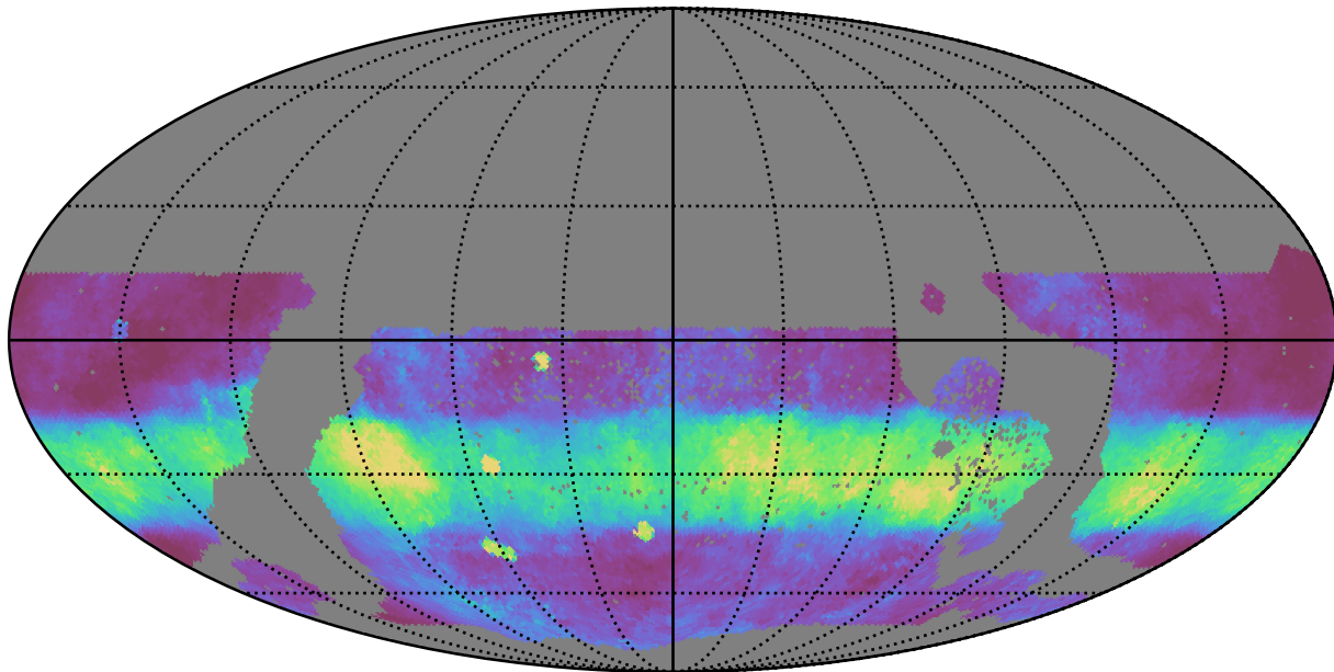
too_elab_r32_d3_gz_v3.4_10yrs WFD r band: Median normairmass
