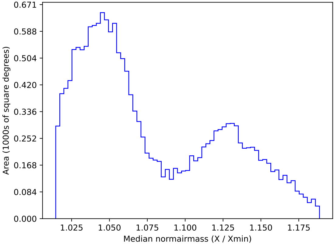
too_elab_r32_d3_gz_v3.4_10yrs WFD r band: Median normairmass
