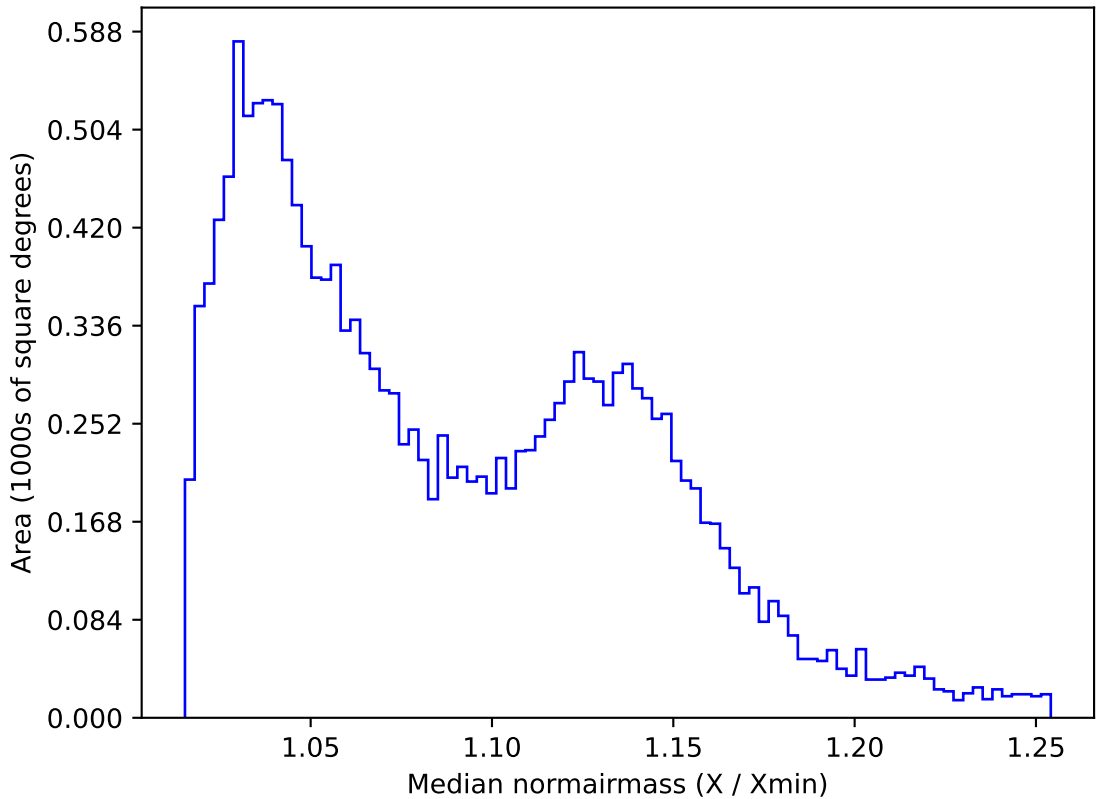
too_elab_r32_d3_gz_v3.4_10yrs WFD g band: Median normairmass
