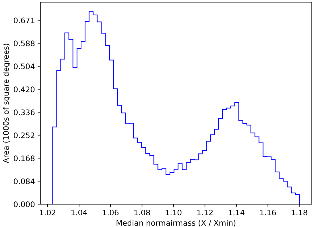
too_elab_r32_d3_gz_v3.4_10yrs WFD all bands: Median normairmass
