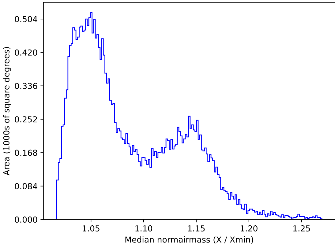
too_elab_r32_d3_gz_v3.4_10yrs All sky z band: Median normairmass
