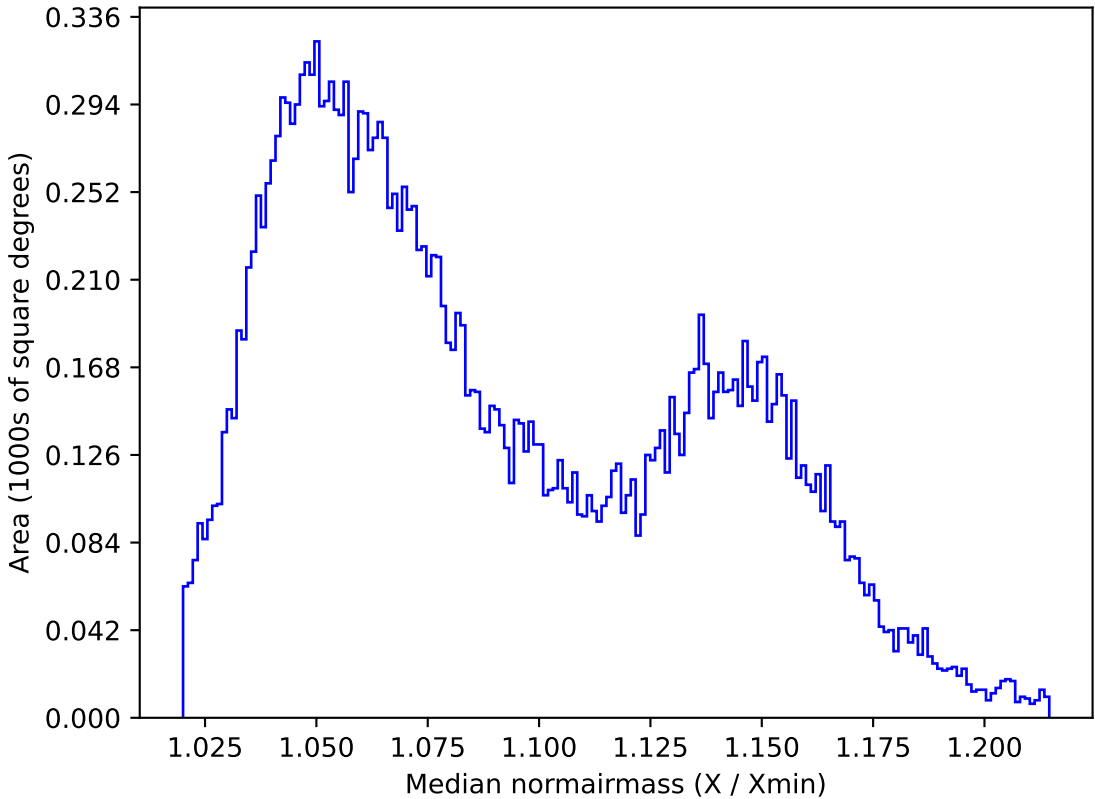
too_elab_r32_d3_gz_v3.4_10yrs All sky y band: Median normairmass
