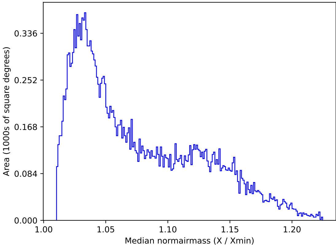
too_elab_r32_d3_gz_v3.4_10yrs All sky u band: Median normairmass
