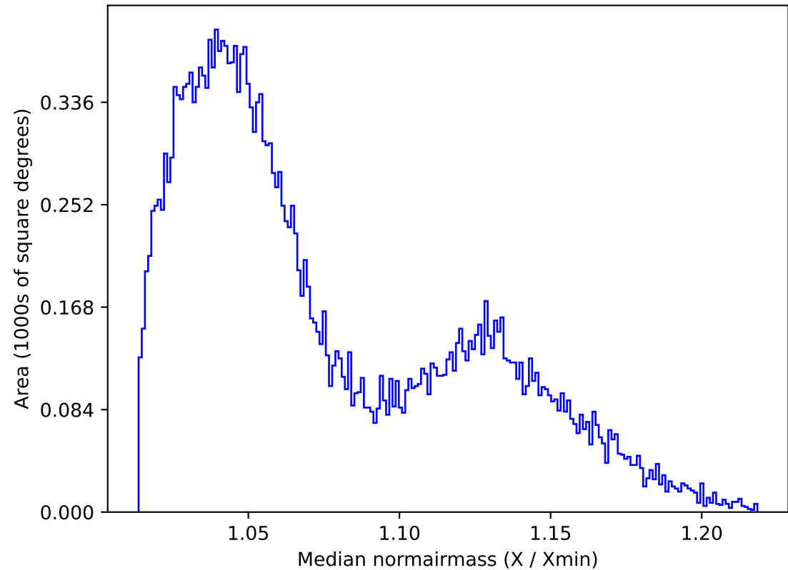
too_elab_r32_d3_gz_v3.4_10yrs All sky r band: Median normairmass
