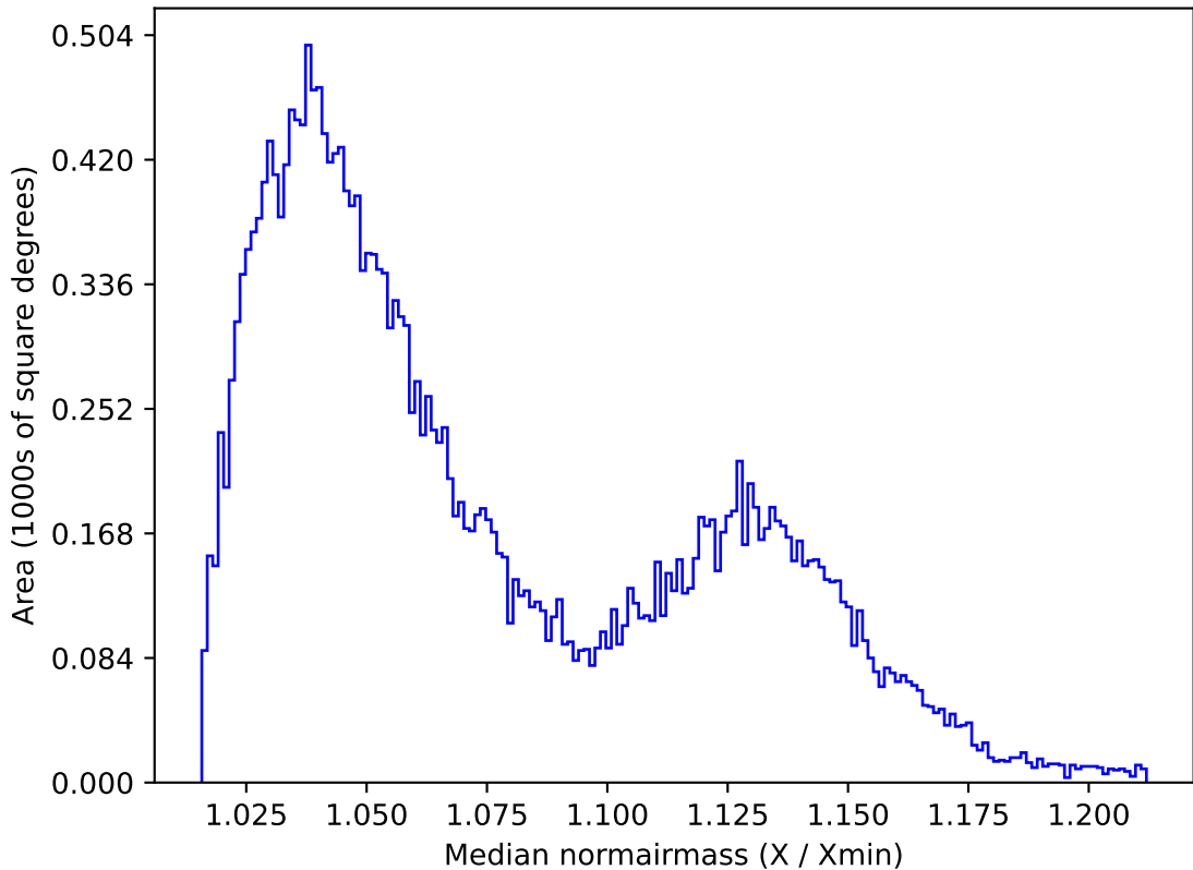
too_elab_r32_d3_gz_v3.4_10yrs All sky i band: Median normairmass
