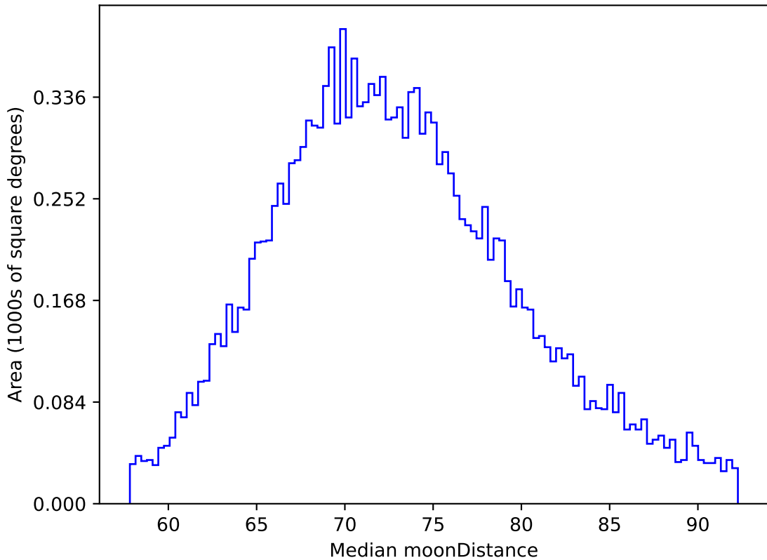
too_elab_r32_d3_gz_v3.4_10yrs WFD z band: Median moonDistance
