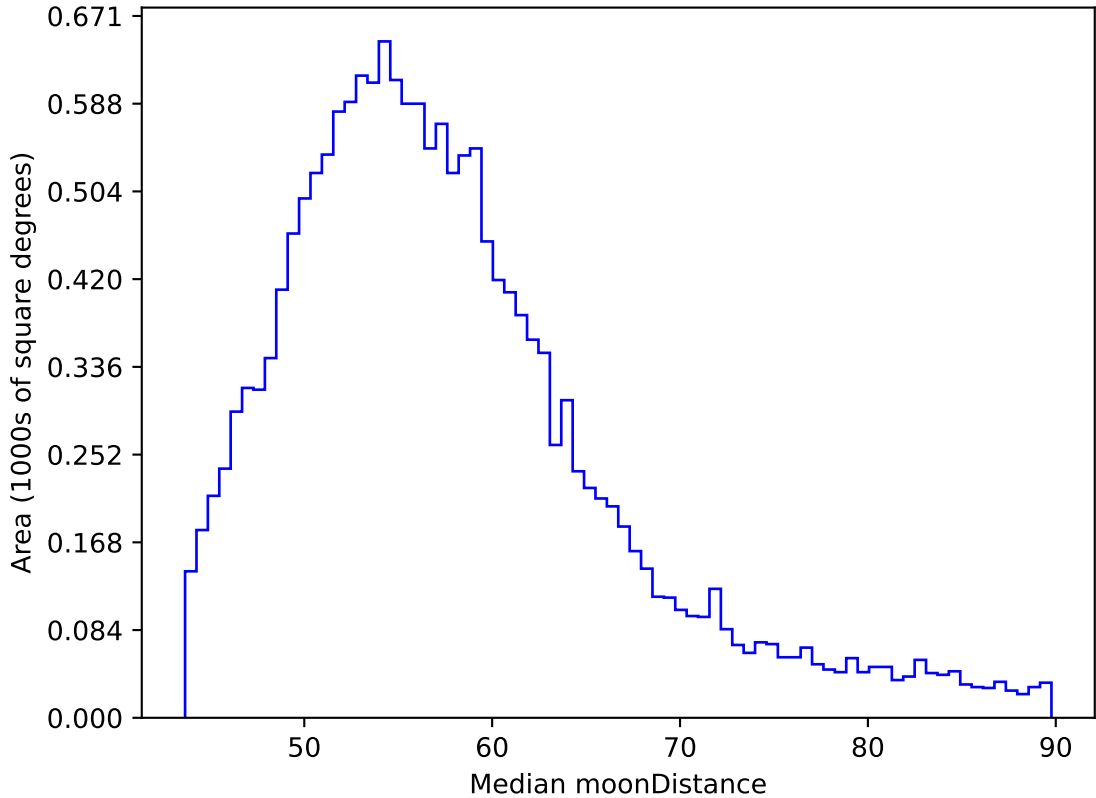
too_elab_r32_d3_gz_v3.4_10yrs WFD y band: Median moonDistance
