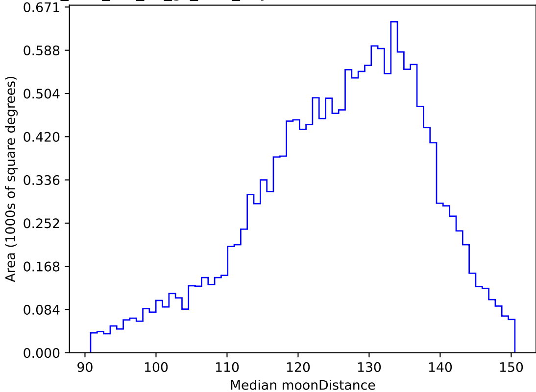
too_elab_r32_d3_gz_v3.4_10yrs WFD u band: Median moonDistance
