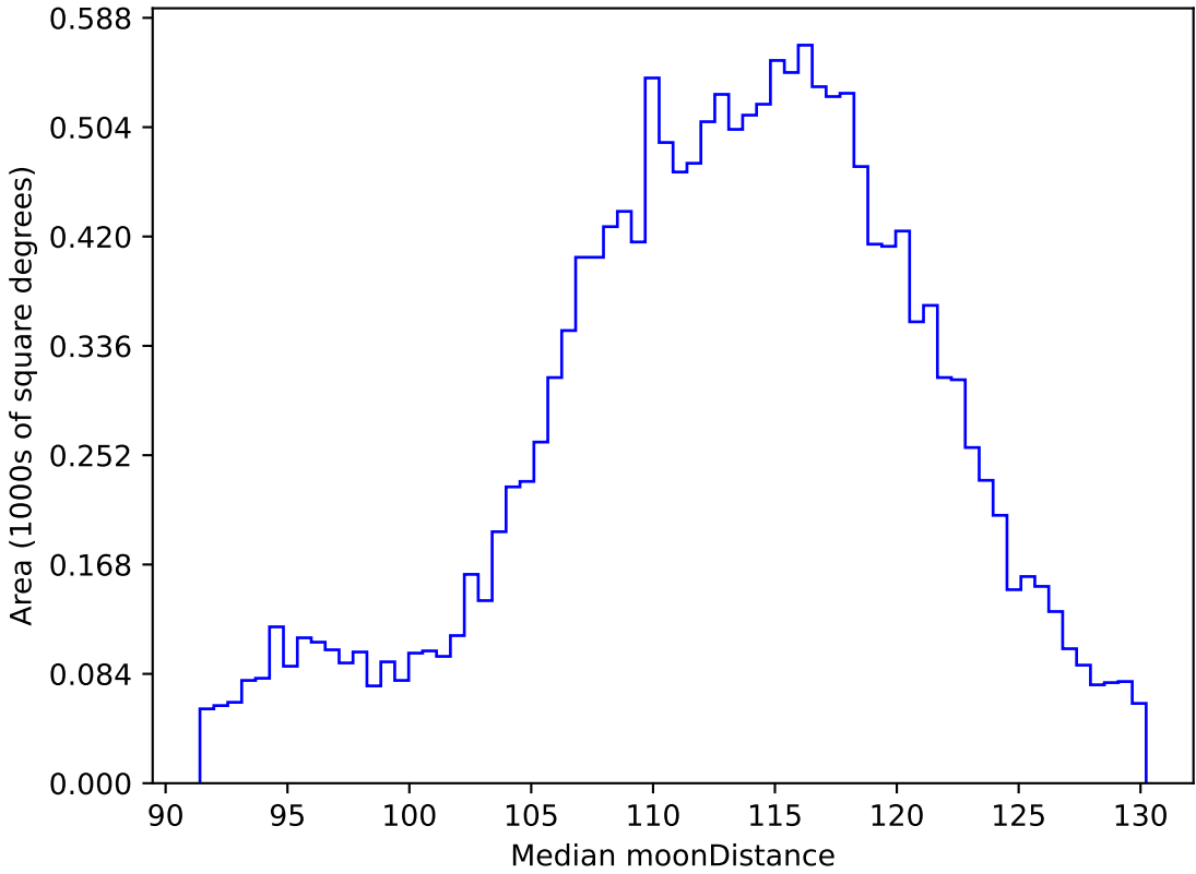
too_elab_r32_d3_gz_v3.4_10yrs WFD r band: Median moonDistance
