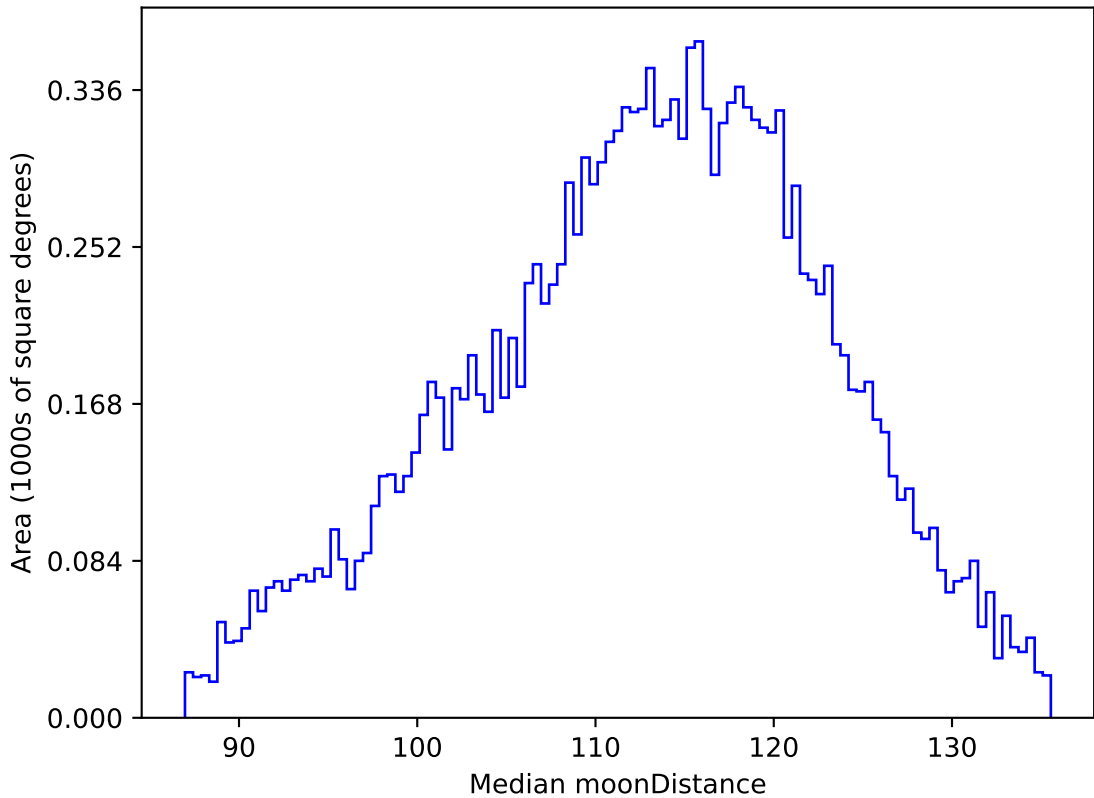
too_elab_r32_d3_gz_v3.4_10yrs WFD g band: Median moonDistance
