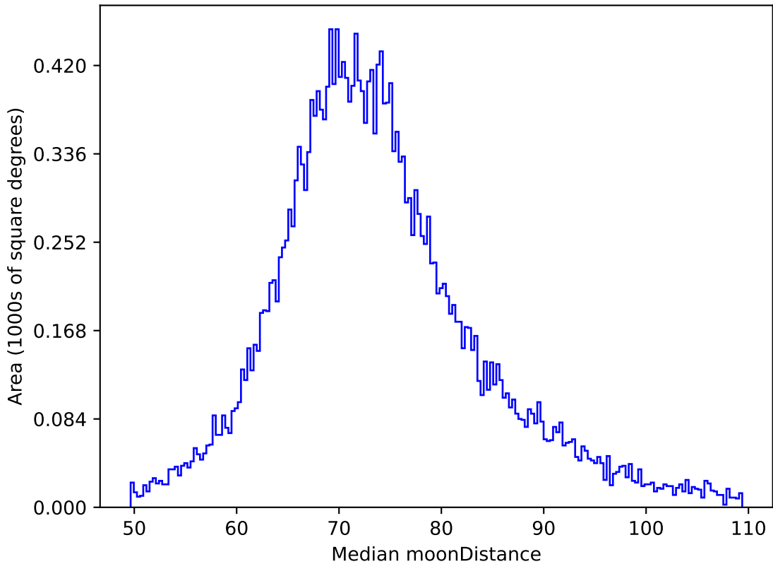
too_elab_r32_d3_gz_v3.4_10yrs All sky z band: Median moonDistance
