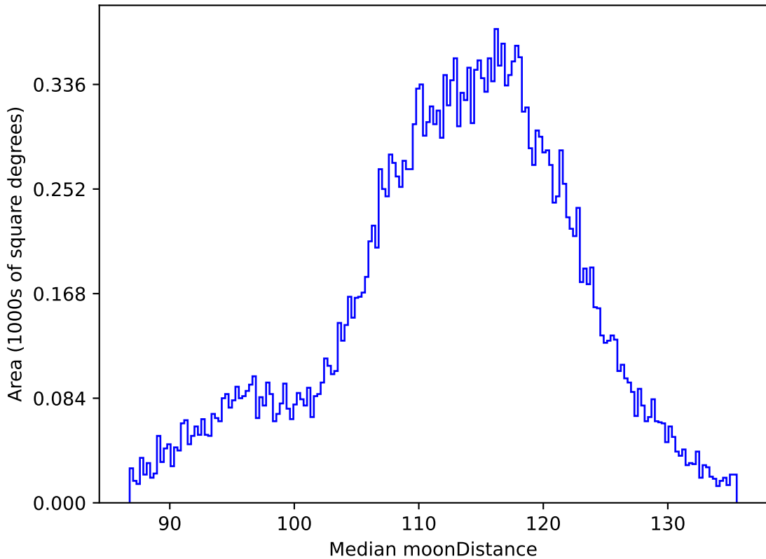
too_elab_r32_d3_gz_v3.4_10yrs All sky r band: Median moonDistance
