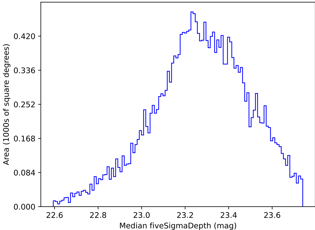
too_elab_r32_d3_gz_v3.4_10yrs Yr 1 u band: Median fiveSigmaDepth
