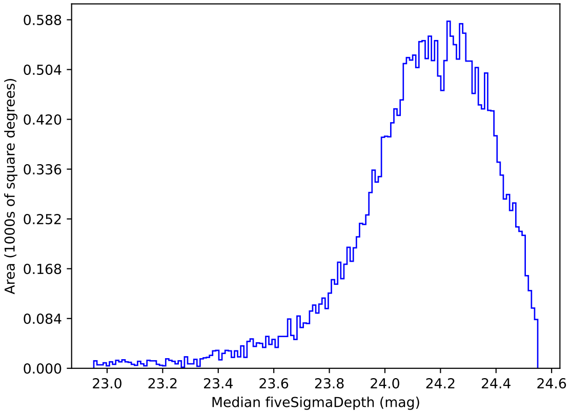
too_elab_r32_d3_gz_v3.4_10yrs Yr 1 r band: Median fiveSigmaDepth
