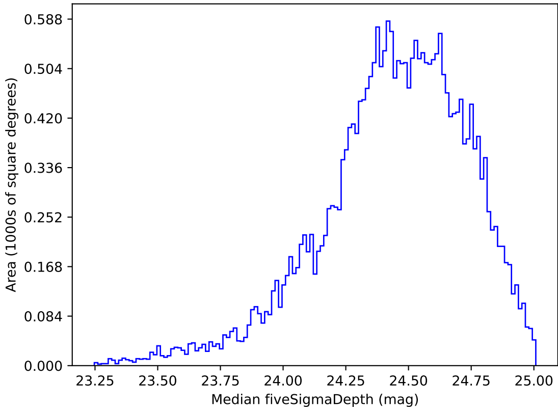
too_elab_r32_d3_gz_v3.4_10yrs Yr 1 g band: Median fiveSigmaDepth
