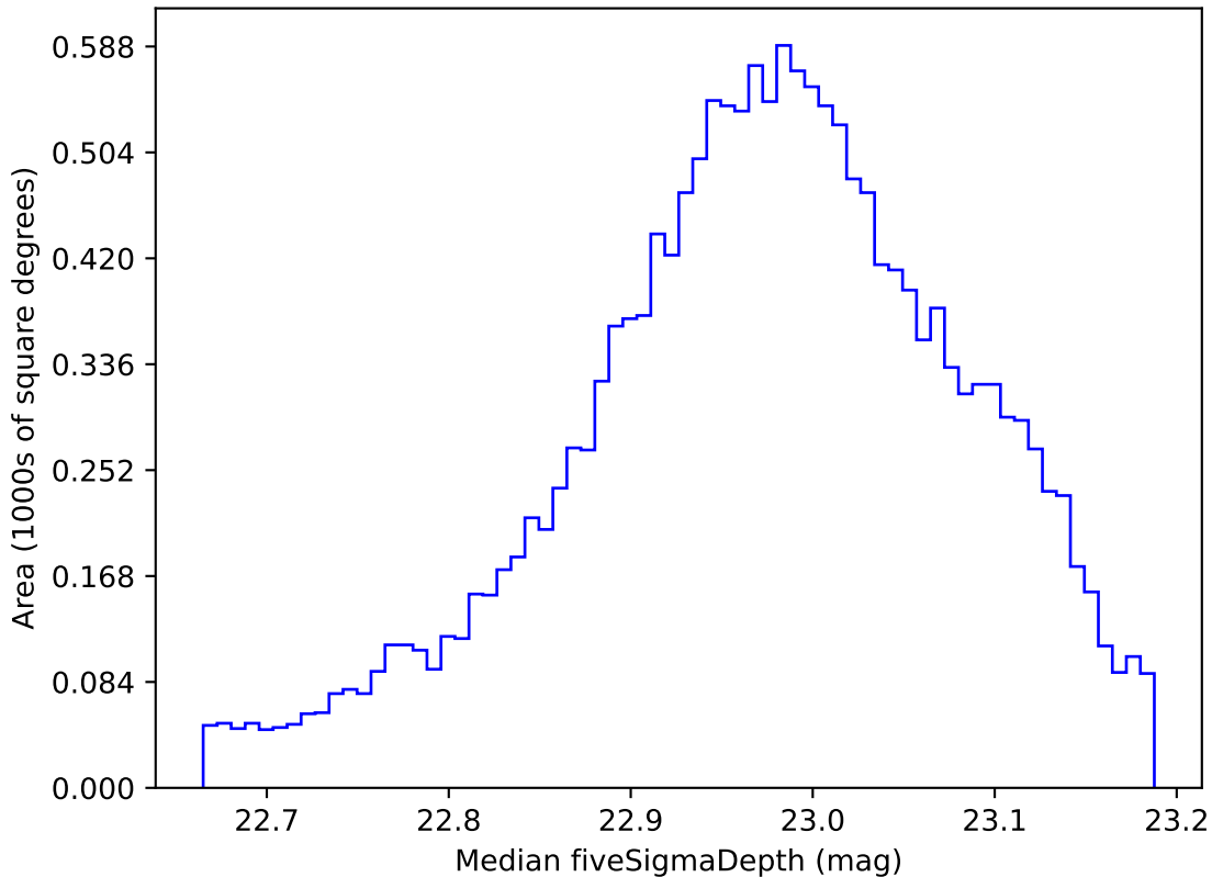
too_elab_r32_d3_gz_v3.4_10yrs WFD z band: Median fiveSigmaDepth
