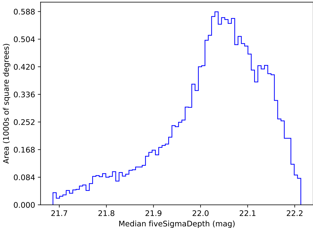
too_elab_r32_d3_gz_v3.4_10yrs WFD y band: Median fiveSigmaDepth
