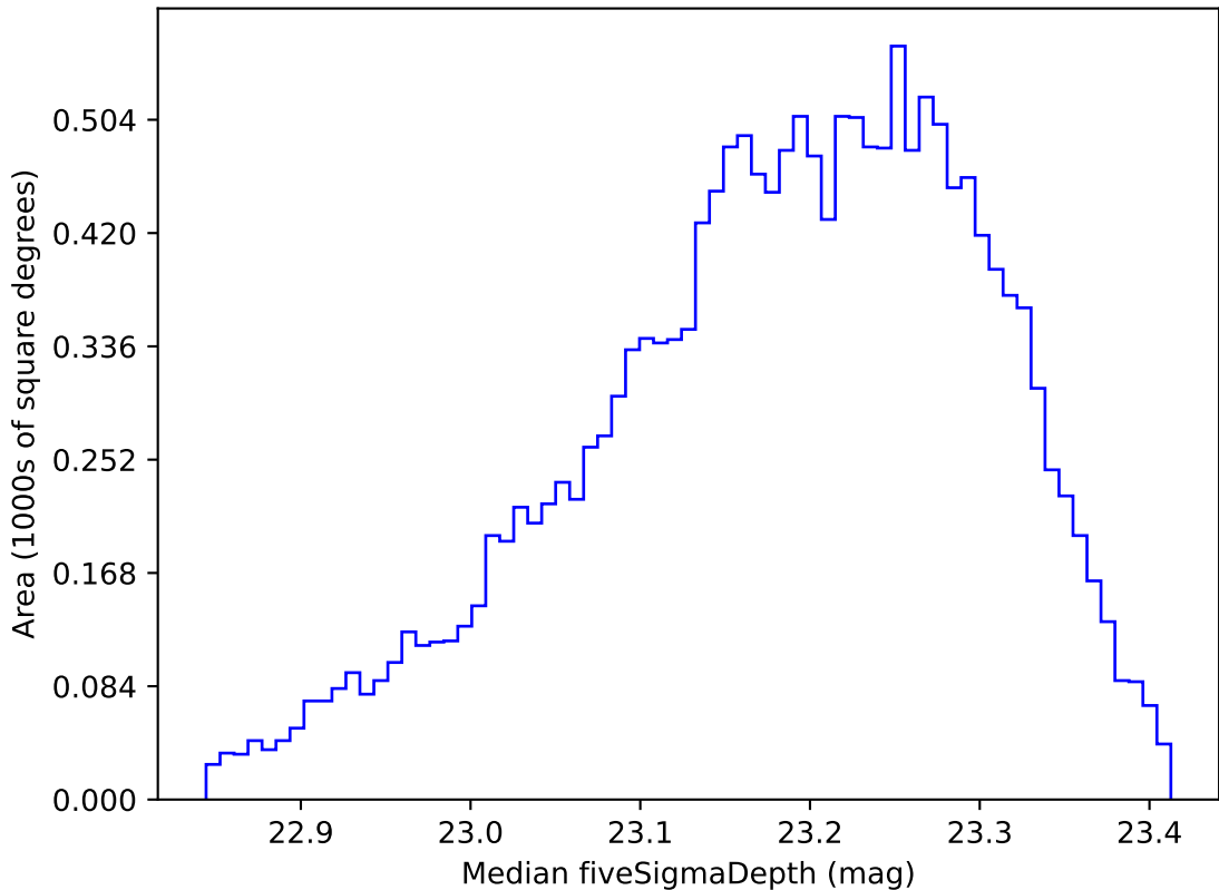
too_elab_r32_d3_gz_v3.4_10yrs WFD u band: Median fiveSigmaDepth
