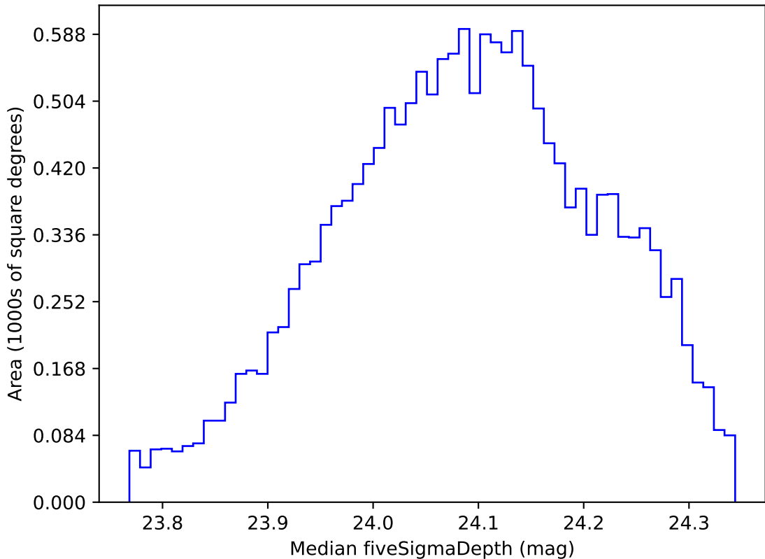
too_elab_r32_d3_gz_v3.4_10yrs WFD r band: Median fiveSigmaDepth
