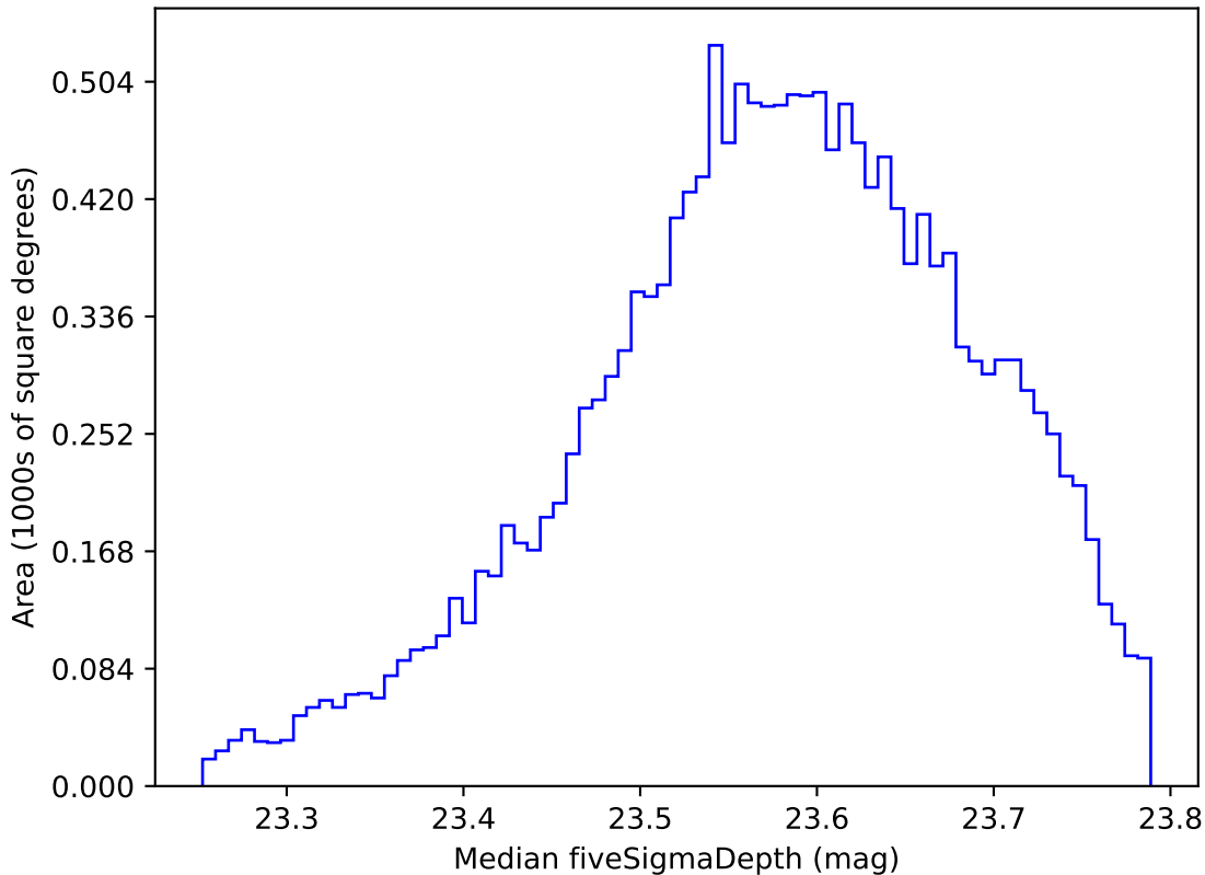
too_elab_r32_d3_gz_v3.4_10yrs WFD i band: Median fiveSigmaDepth
