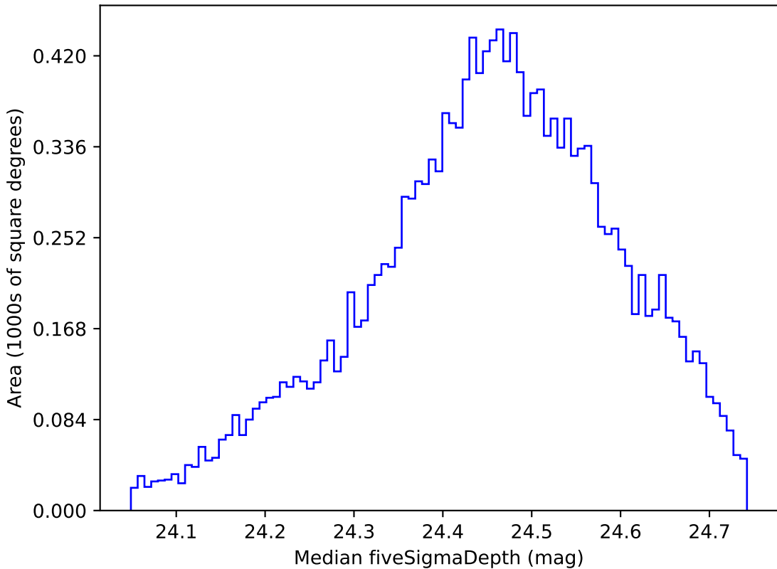
too_elab_r32_d3_gz_v3.4_10yrs WFD g band: Median fiveSigmaDepth
