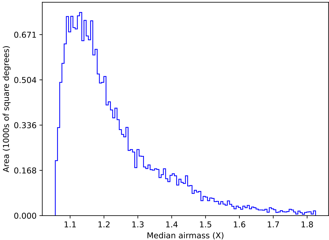
too_elab_r32_d3_gz_v3.4_10yrs Yr 1 u band: Median airmass
