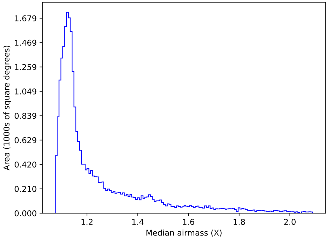
too_elab_r32_d3_gz_v3.4_10yrs Yr 1 all bands: Median airmass
