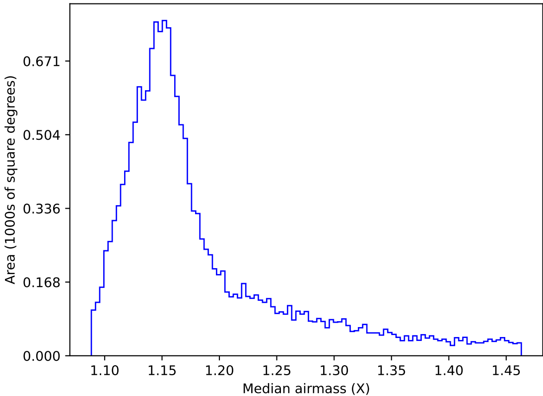
too_elab_r32_d3_gz_v3.4_10yrs WFD z band: Median airmass
