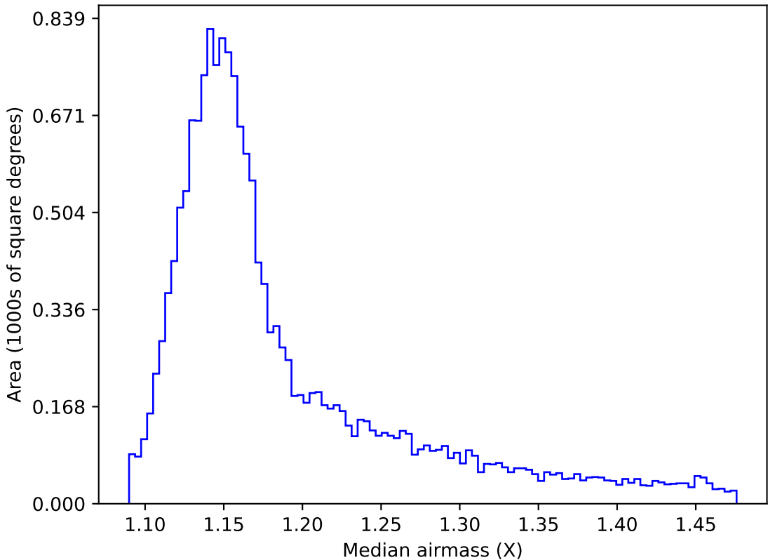
too_elab_r32_d3_gz_v3.4_10yrs WFD y band: Median airmass
