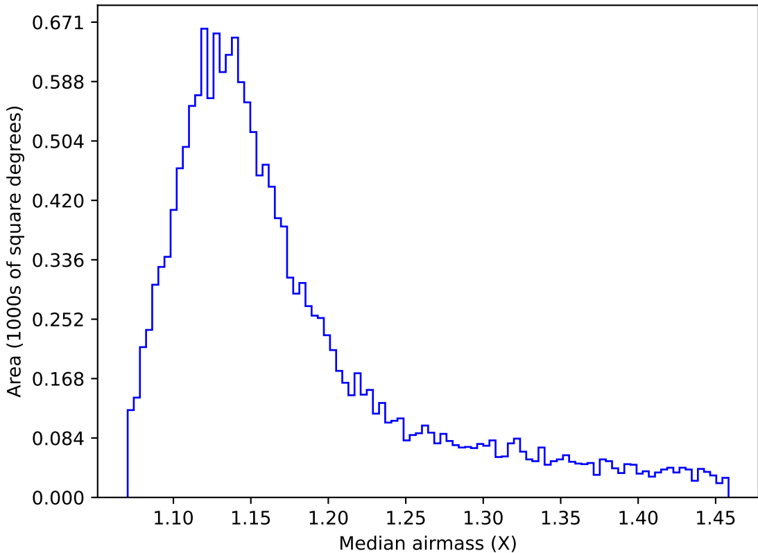
too_elab_r32_d3_gz_v3.4_10yrs WFD u band: Median airmass
