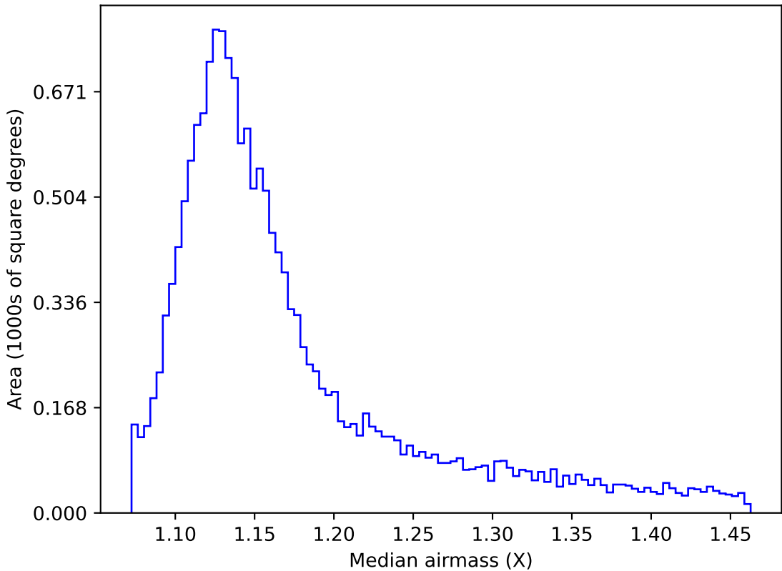
too_elab_r32_d3_gz_v3.4_10yrs WFD r band: Median airmass
