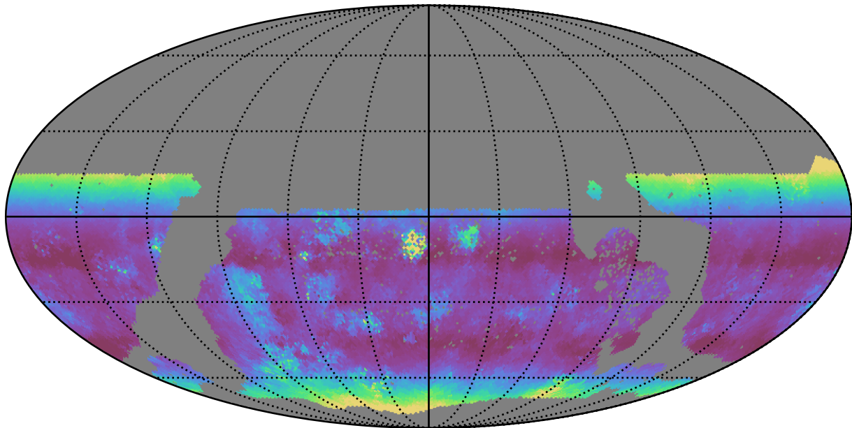
too_elab_r32_d3_gz_v3.4_10yrs WFD g band: Median airmass
