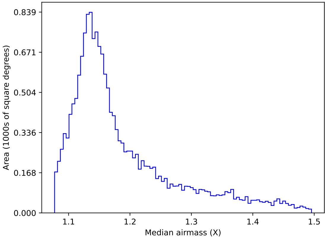
too_elab_r32_d3_gz_v3.4_10yrs WFD g band: Median airmass
