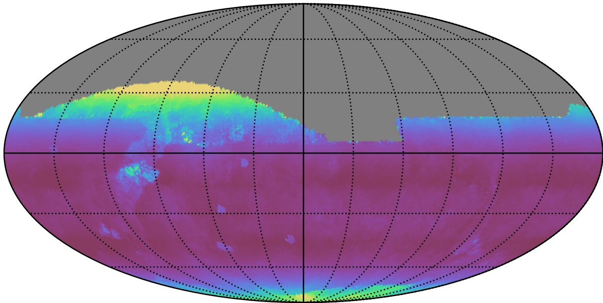
too_elab_r32_d3_gz_v3.4_10yrs All sky z band: Median airmass
