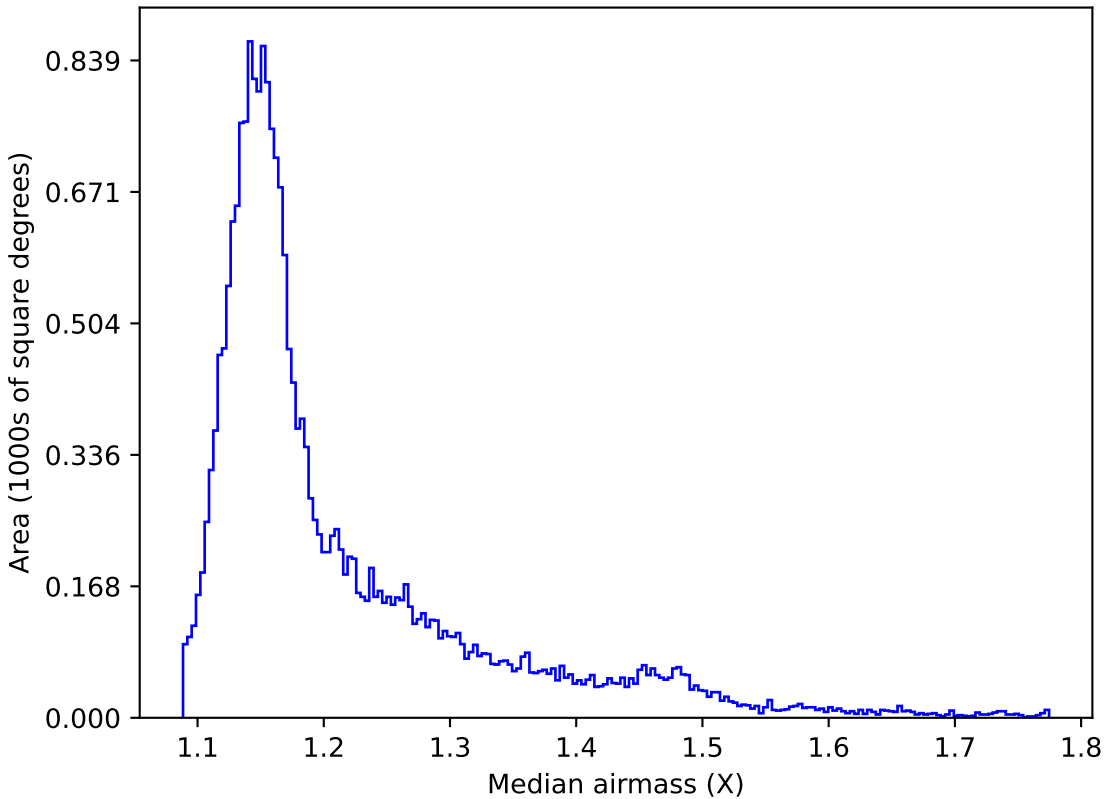
too_elab_r32_d3_gz_v3.4_10yrs All sky y band: Median airmass
