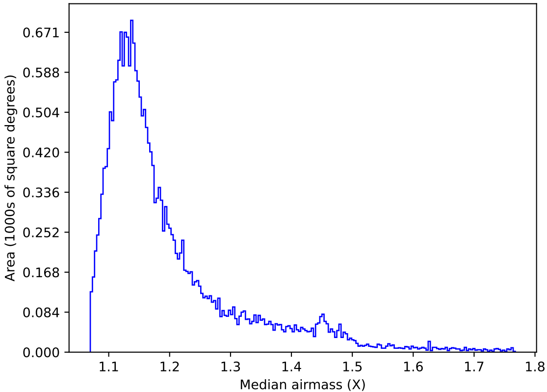
too_elab_r32_d3_gz_v3.4_10yrs All sky u band: Median airmass
