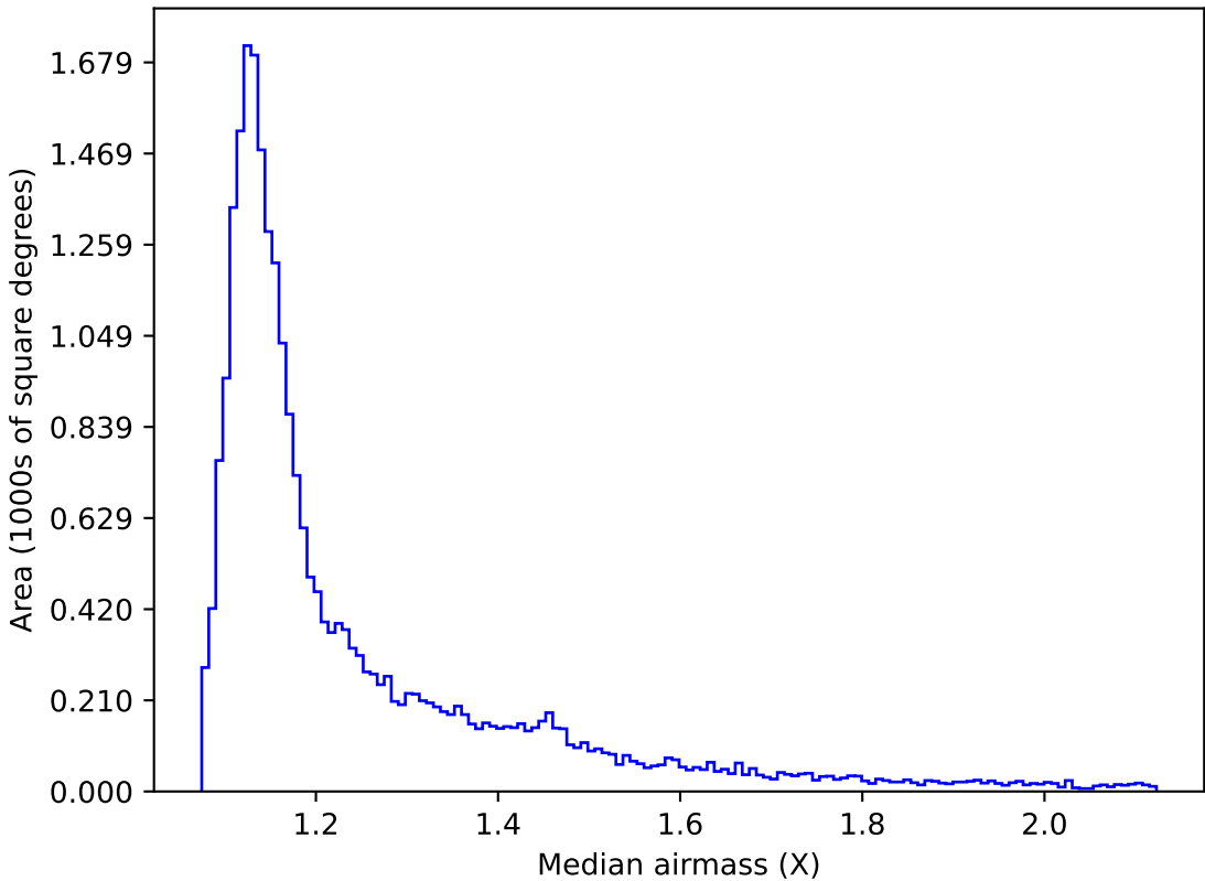
too_elab_r32_d3_gz_v3.4_10yrs All sky r band: Median airmass
