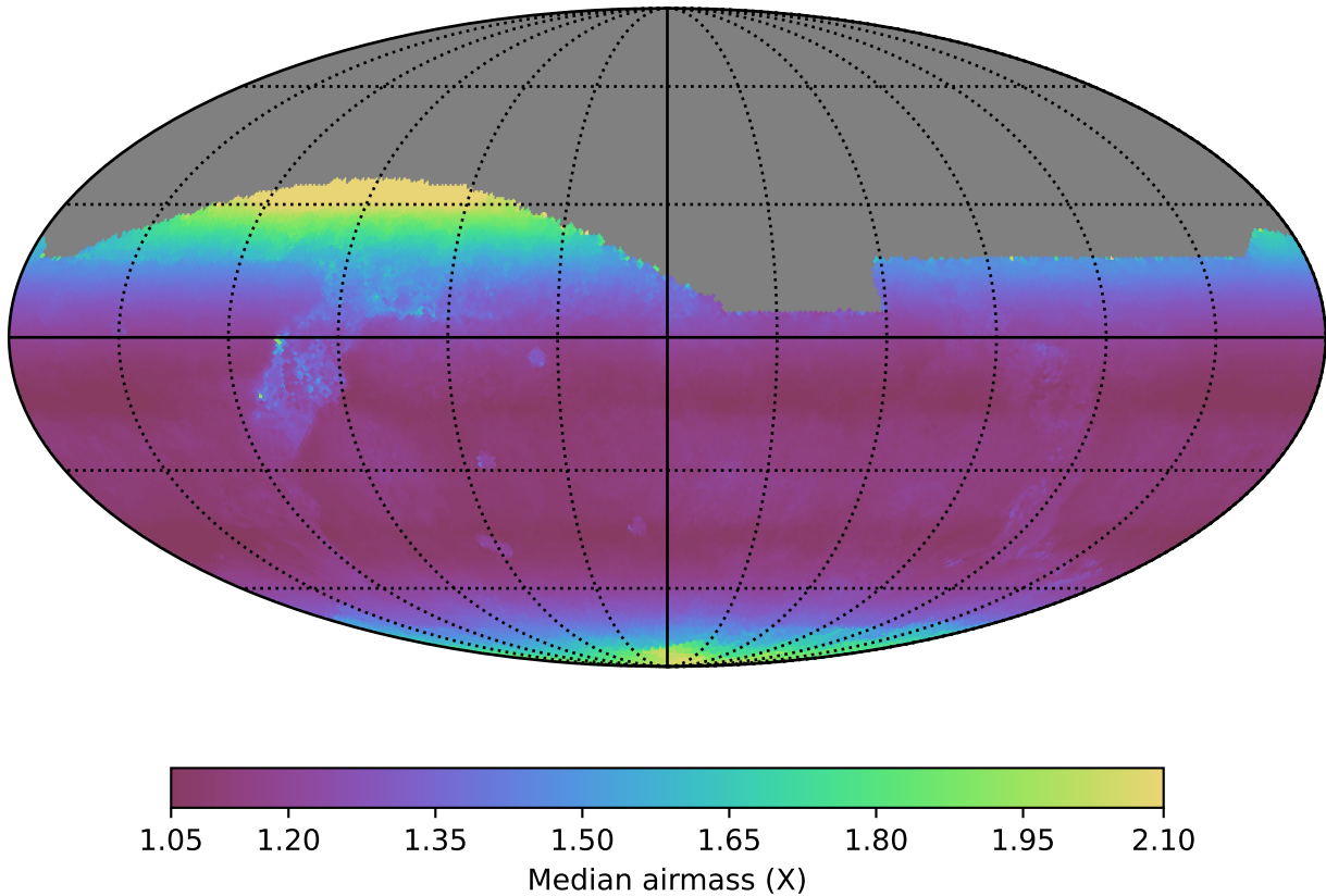
too_elab_r32_d3_gz_v3.4_10yrs All sky i band: Median airmass
