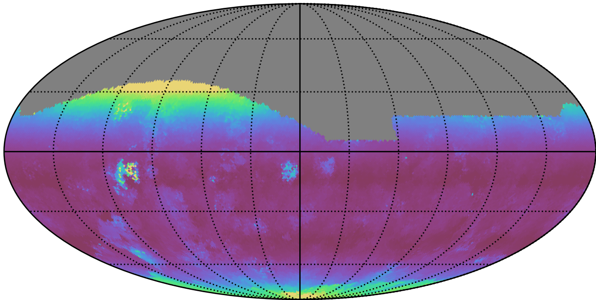
too_elab_r32_d3_gz_v3.4_10yrs All sky g band: Median airmass
