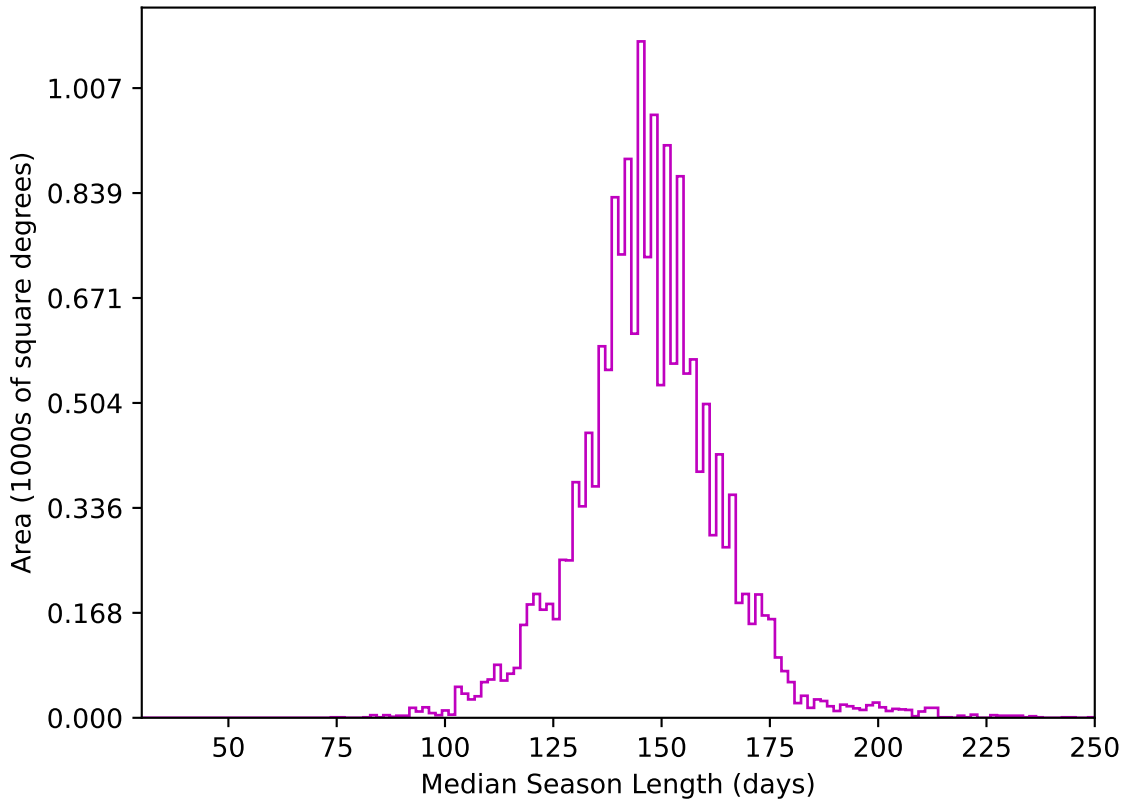
too_elab_r32_d3_gz_v3.4_10yrs WFD z band: Median Season Length
