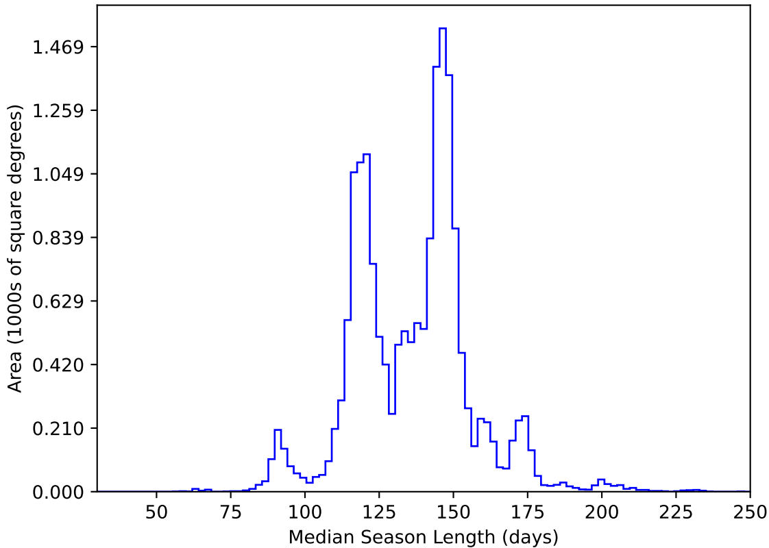
too_elab_r32_d3_gz_v3.4_10yrs WFD y band: Median Season Length
