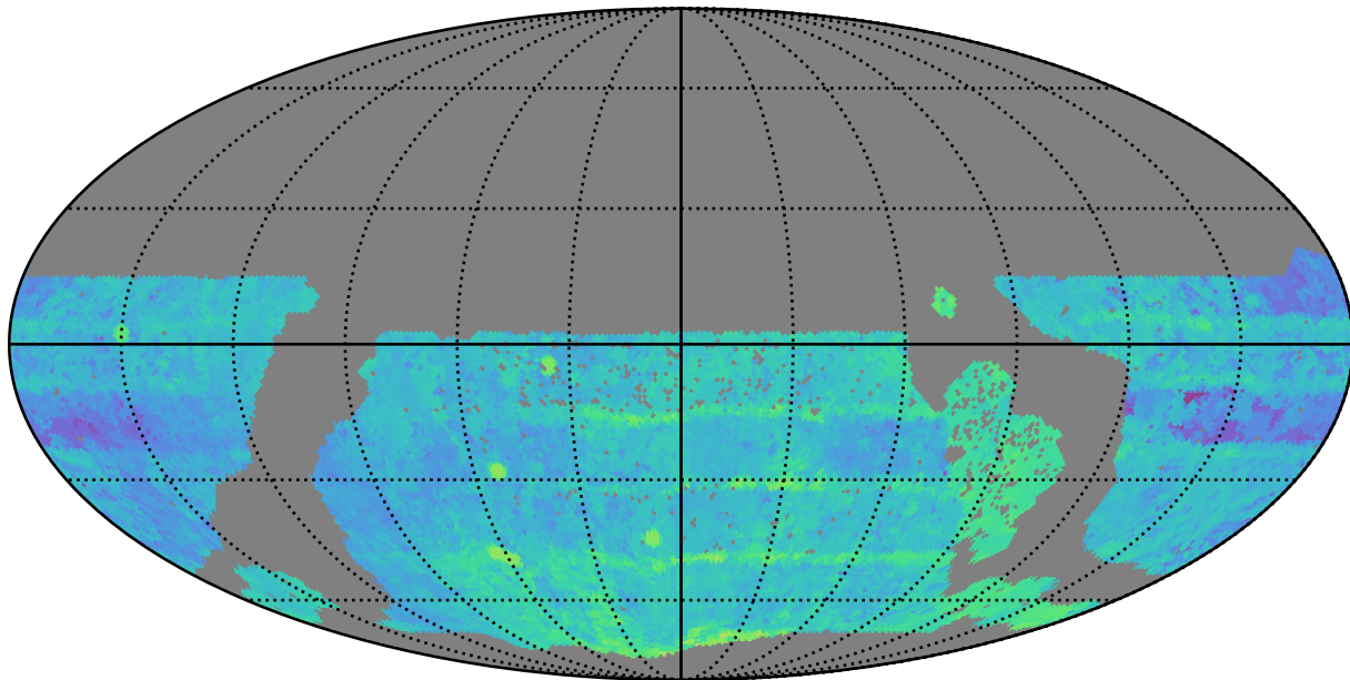
too_elab_r32_d3_gz_v3.4_10yrs WFD r band: Median Season Length
