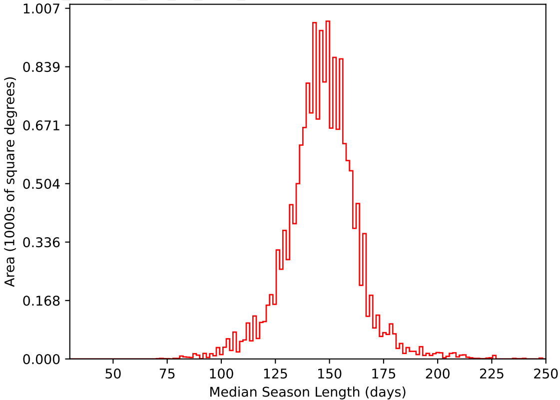
too_elab_r32_d3_gz_v3.4_10yrs WFD i band: Median Season Length
