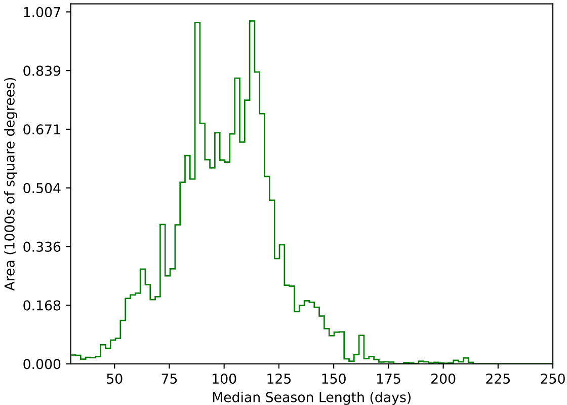
too_elab_r32_d3_gz_v3.4_10yrs WFD g band: Median Season Length
