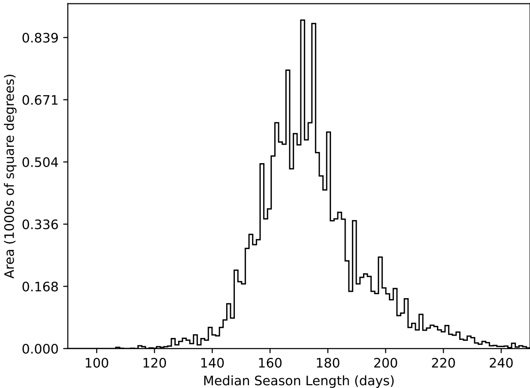
too_elab_r32_d3_gz_v3.4_10yrs WFD all bands: Median Season Length
