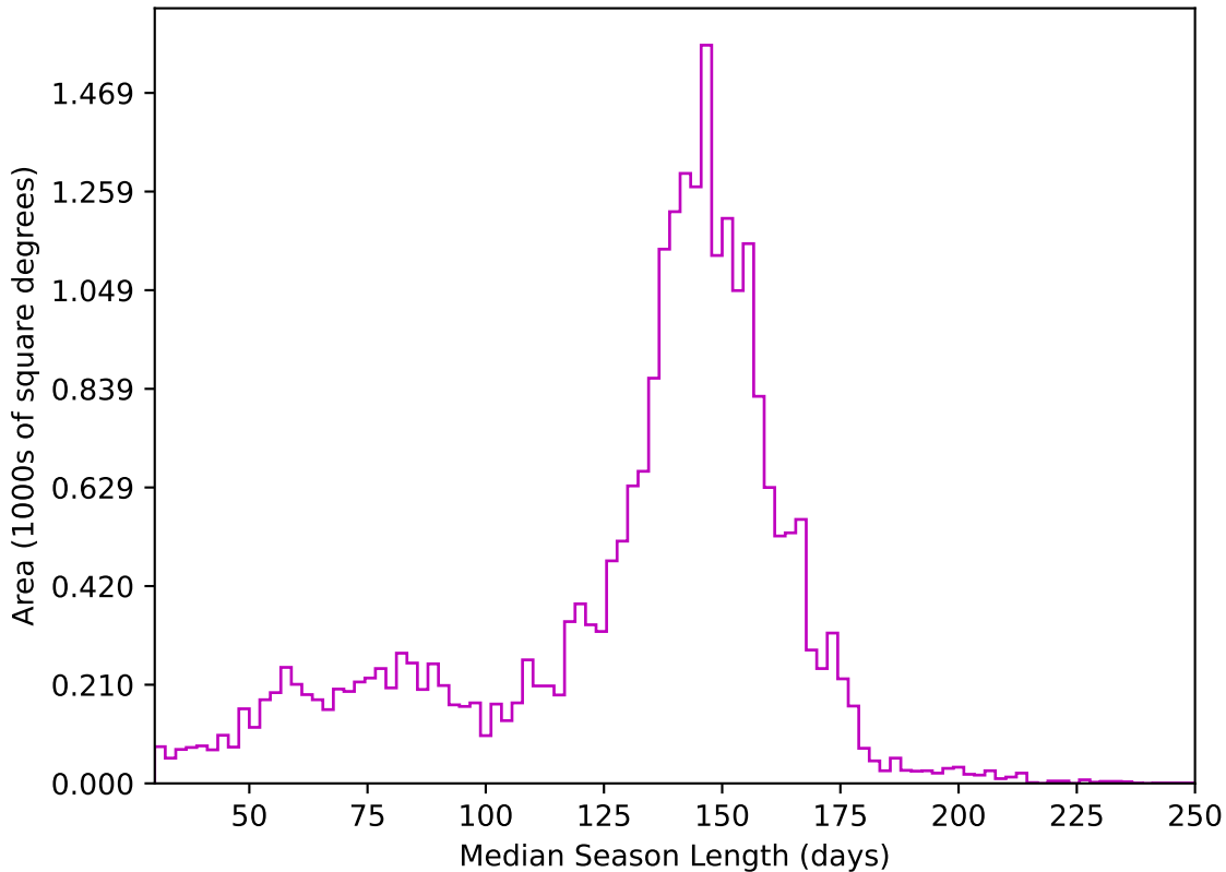
too_elab_r32_d3_gz_v3.4_10yrs All sky z band: Median Season Length
