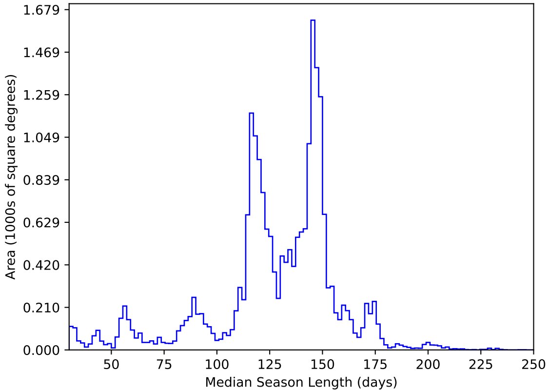
too_elab_r32_d3_gz_v3.4_10yrs All sky y band: Median Season Length
