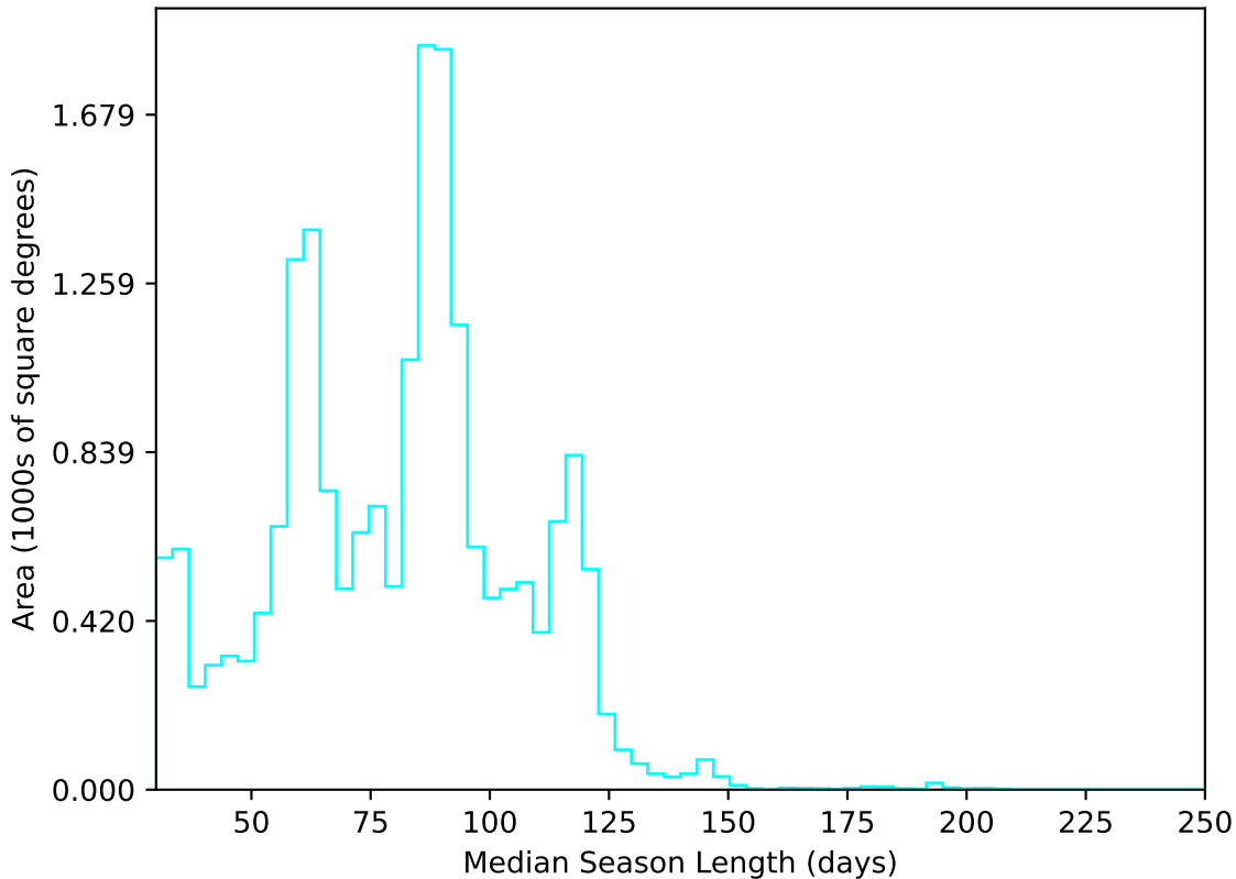
too_elab_r32_d3_gz_v3.4_10yrs All sky u band: Median Season Length
