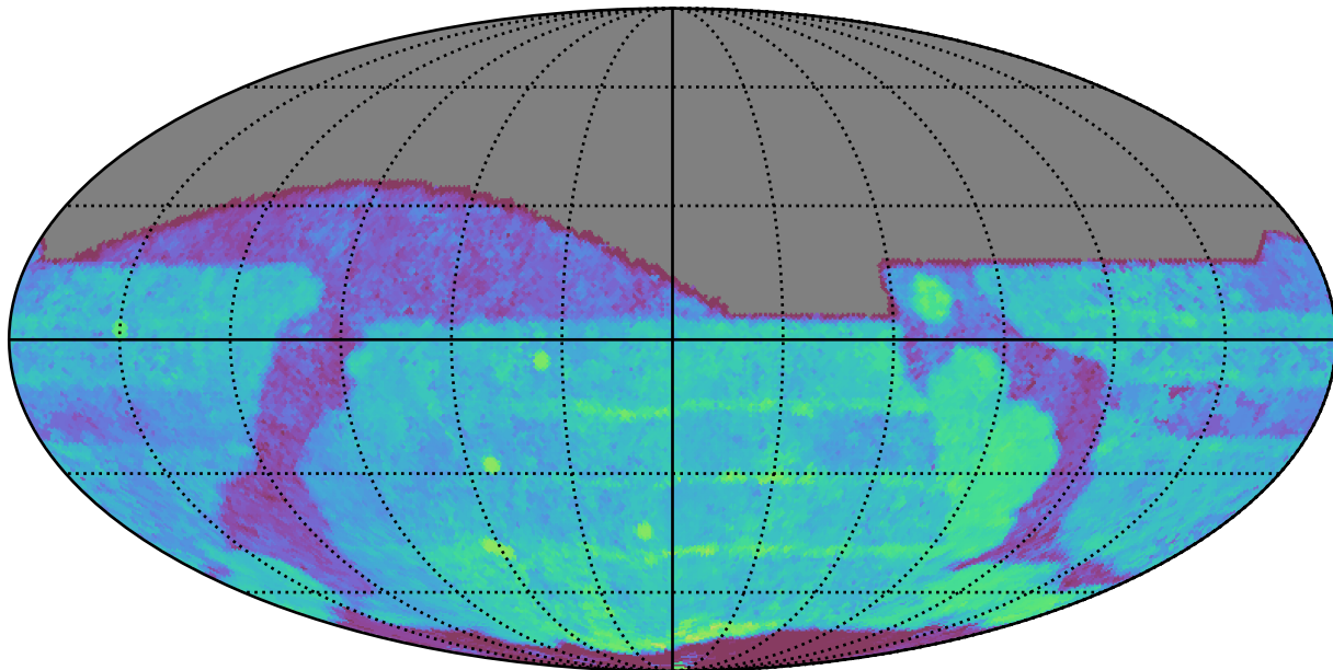
too_elab_r32_d3_gz_v3.4_10yrs All sky r band: Median Season Length
